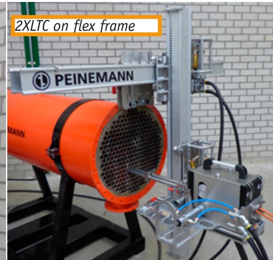
2XLTC in vertical setup
